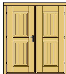
T28-DT-G Madriers de: 28 mm masse: 150 x 184 cm
